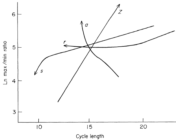
FIG. 2. Analysis of the limit cycle in May's (1973) model, eqn (1). This figure illustrates changes in cycle length and the ratio of the maximum over minimum prey population size as a function of changes in four parameters, Z = K/D , a = cq , r and s . For further explanations and the parameter values see Table 2. The four lines were drawn through the average points for the respective parameters, calculated over all possible combinations of the values of other parameters. Cycle length has arbitrary units.
