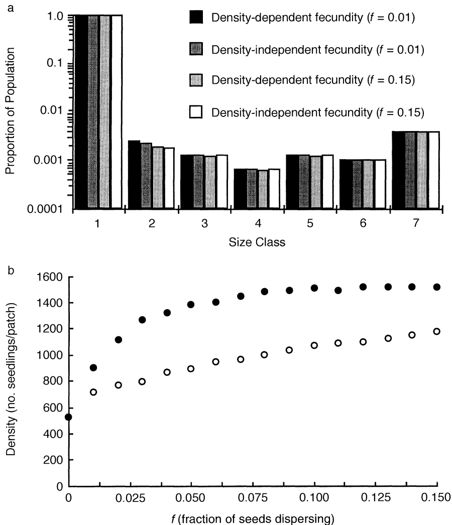
FIG. 8. Effects of density-dependent fecundity on predictions of stable size distributions and equilibrium densities. (a) The equilibrium stable size distributions when seedling production ( n_7 F_7 ) is set at a constant (i.e., is density dependent), compared with those predicted when seedling production is a function of adult density (i.e., is density independent). The fraction of seeds dispersing from the natal patch ( f ), was set at a low value ( f = 0.01 ) or a high value ( f = 0.15 ). (b) The equilibrium densities in a 7-m 2 patch when seedling production ( F_7 ) is set at a constant (○) (i.e., is density dependent), compared with those predicted when seedling production is a function of adult density (●) (i.e., is density independent), shown as a function of f , the fraction of seeds dispersing from the natal patch.
