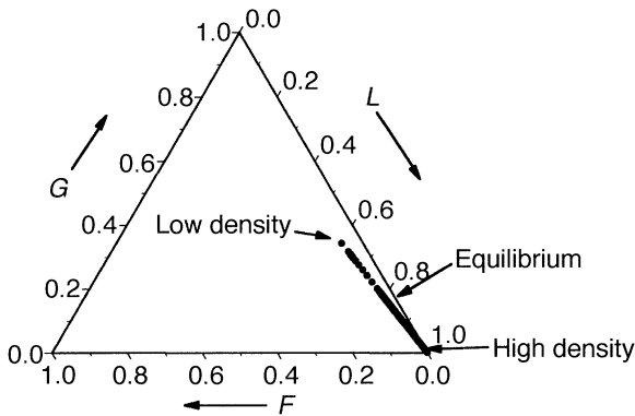
FIG. 5. G - L - F triangular ordination of the population growth elasticities, derived from the density-dependent transition matrix (see Table 2) with P_7 = 0.95 , when populations were allowed to grow from low densities to an equilibrium. G = growth, L = survival, F = fecundity.
