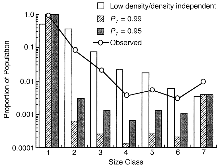
FIG. 2. Observed and simulated size class distributions. Bars indicate the size distributions predicted from the mean transition matrix with P_7 = 0.95 or 0.99 (see Table 2), when population growth is density independent (i.e., with G_1 set at its maximum, density-independent value), as compared with the patterns predicted when population growth is density dependent. The points indicate the mean size distribution across the three years of study.
