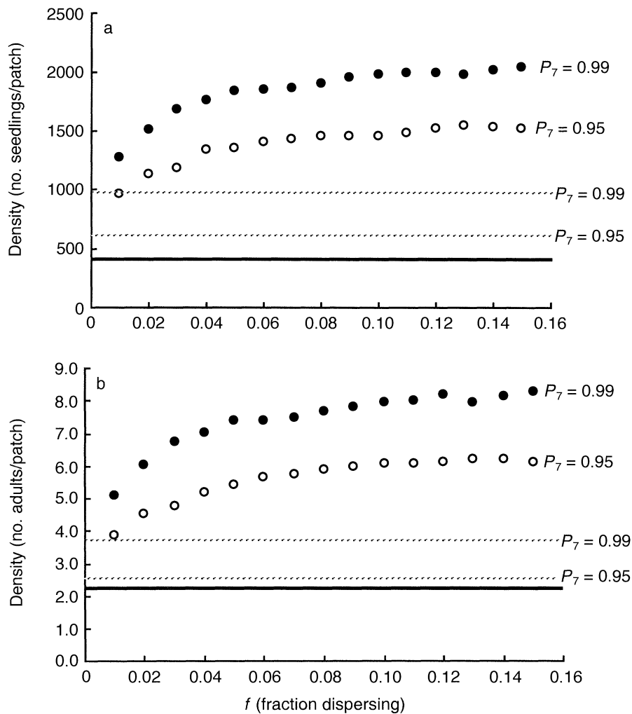
FIG. 7. Effects of changing the dispersal fraction on the equilibrium mean density in a 7-m 2 patch of (a) seedlings and (b) adults in the spatial simulation model, and a comparison with equilibrium densities predicted by the density-dependent form of the mean-density model. The equilibrium densities predicted by the spatial simulation with P_7 set at 0.99 (●) and 0.95 (○) are shown. The horizontal dotted lines show the corresponding predictions of the nonspatial density-dependent model with P_7 set at 0.95 or 0.99 (see Table 2). The solid horizontal lines show the maximum densities recorded in plots during the period of study.
